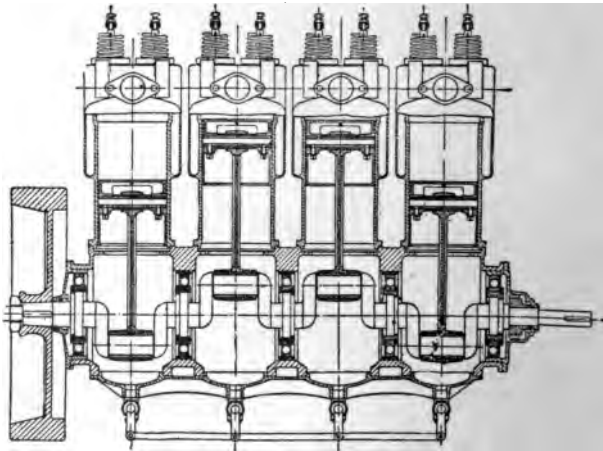
FIG. 391.—Four-cylinder Gasoline Engine, showing the radial ball bearings on the crank shaft.
